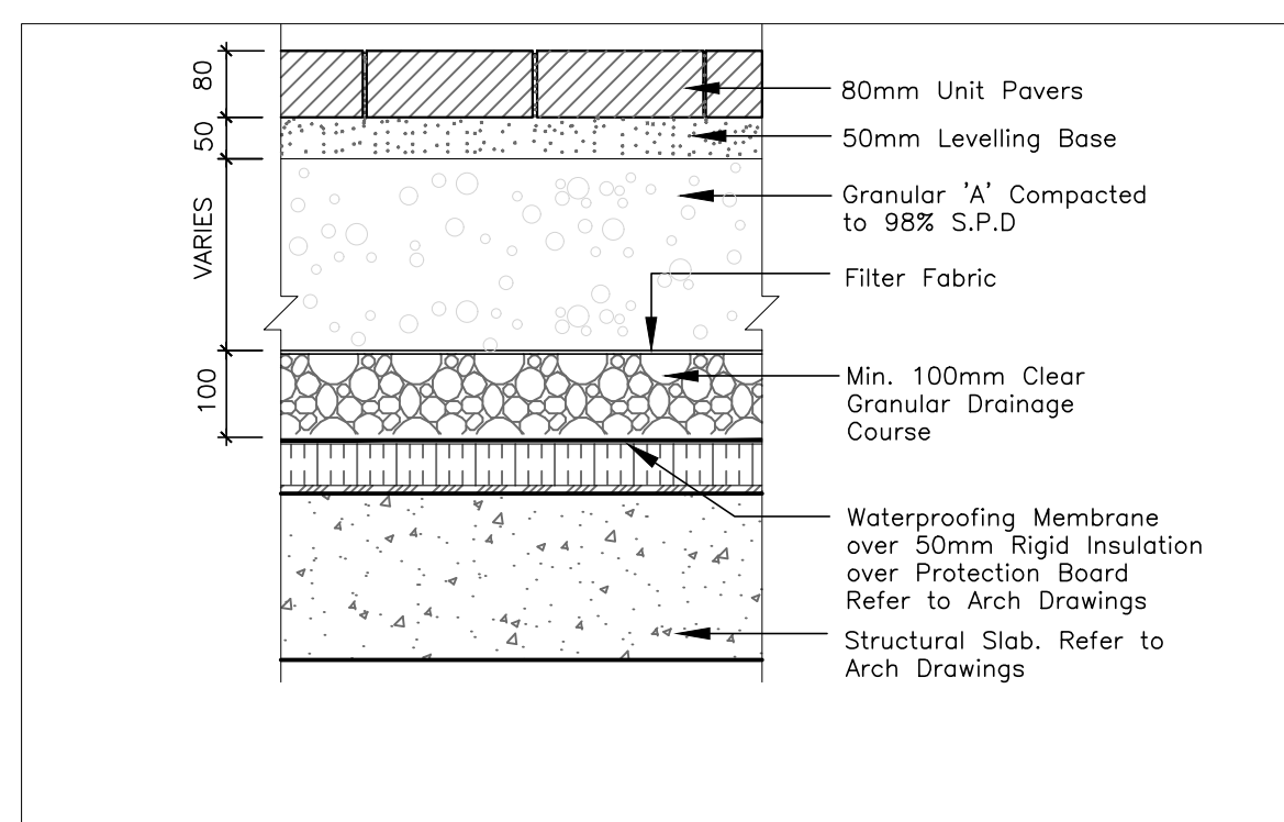
6 TYP. HEAVY DUTY UNIT PAVING ON SLAB L-3.0 1:10
