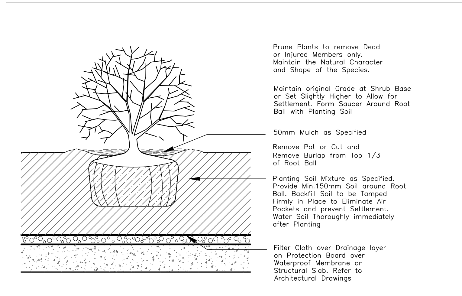
2 TYP. SHRUB PLANTING ON GRADE L-3.0 N.T.S
