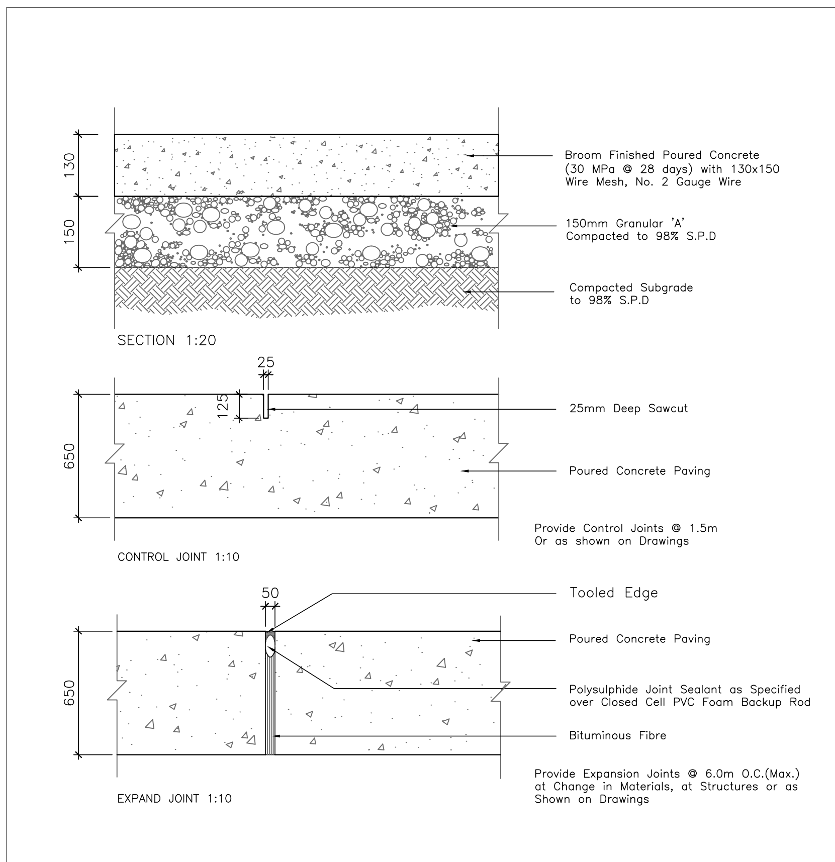
4 TYP. CONCRETE PAVING L-3.0 1:5
