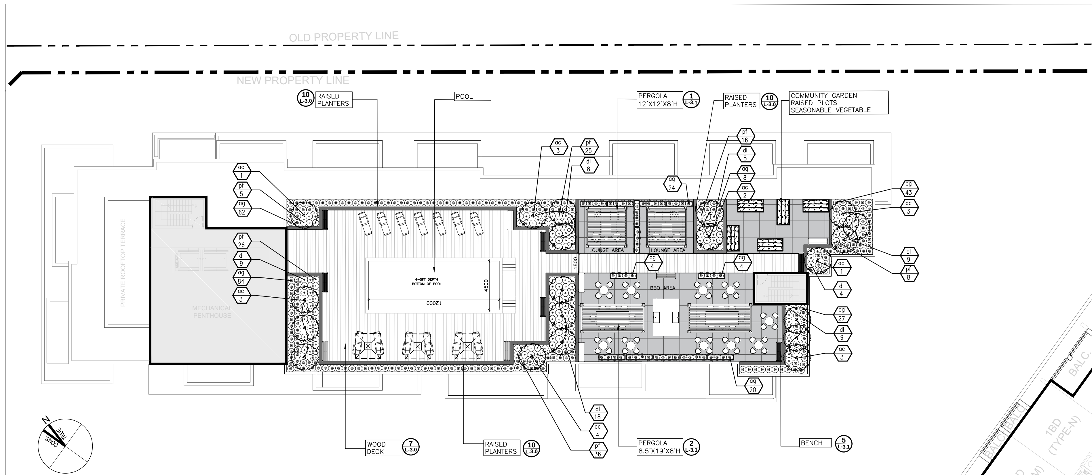
3 PROPOSED LANDSCAPE PLAN ROOF AMENITY-9TH FLOOR L-2.0 1:250
