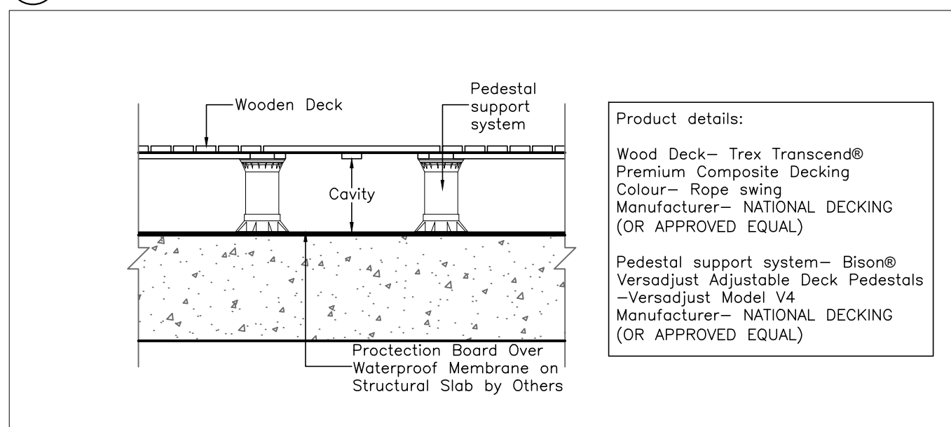
7 TYP. WOOD DECK L-3.0 1:10
