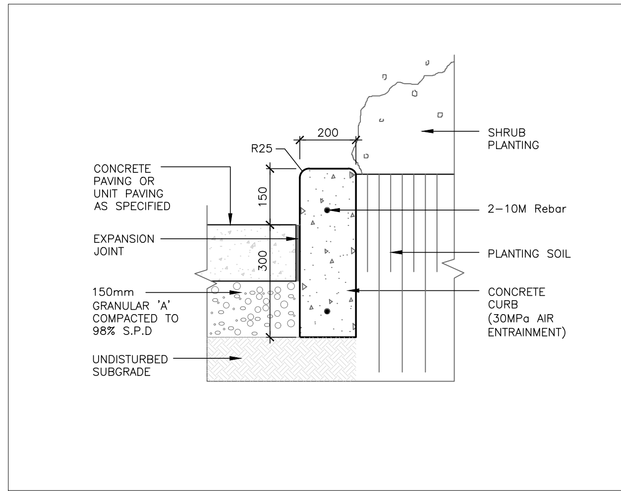
7 PLANTING CURB L-2.0 1:10
