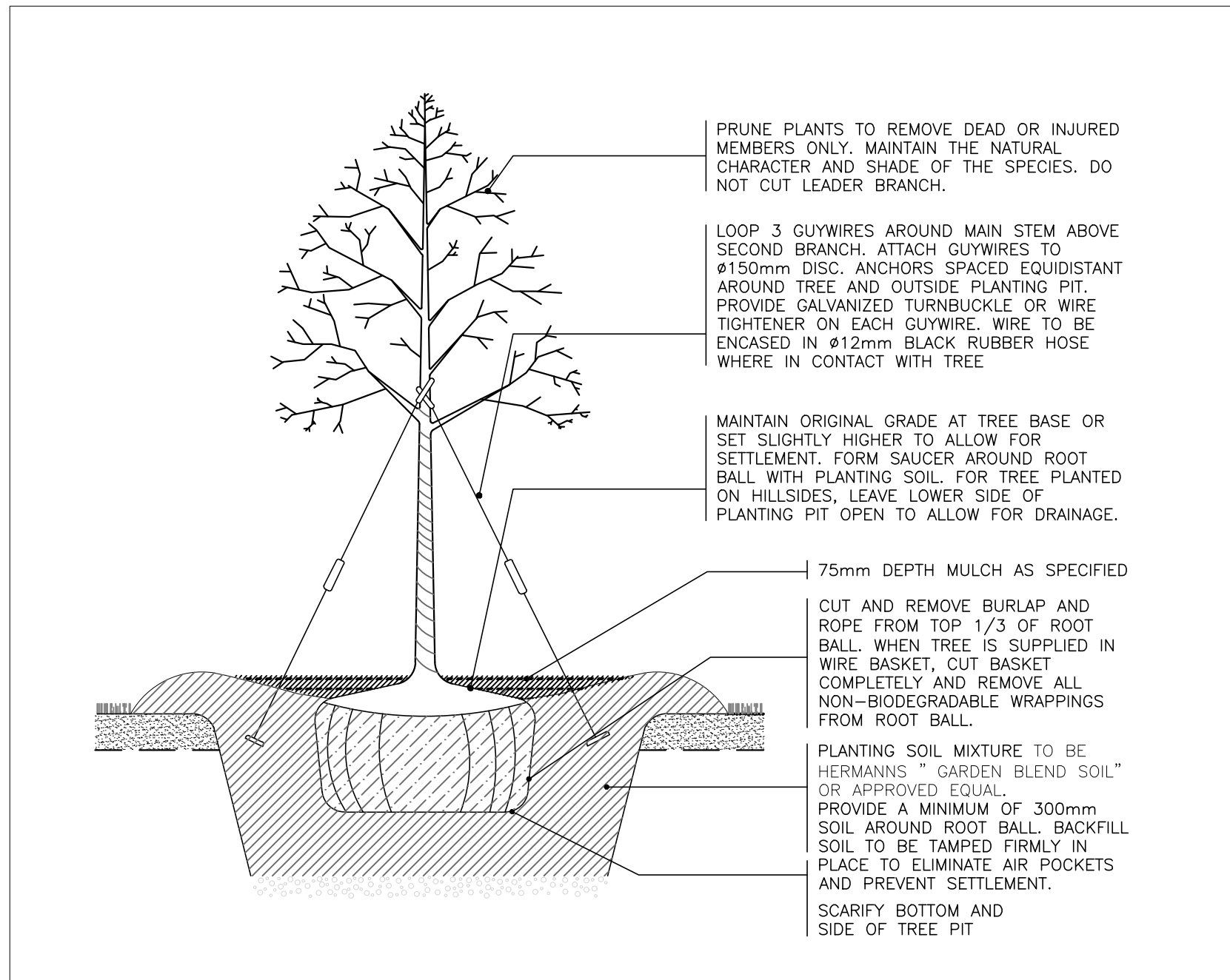
1 TYP. DECIDUOUS TREE PLANTING L-3.0 1:25
