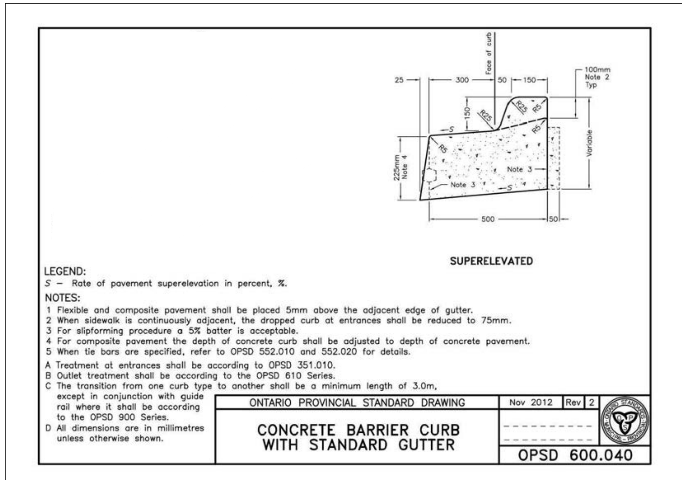
9 FLUSH CURB & BARRIER CURB (SUPERELEVATED) L-3.0 1:10
