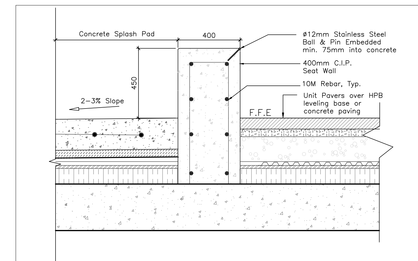
6 SEAT WALL L-3.2 NTS
