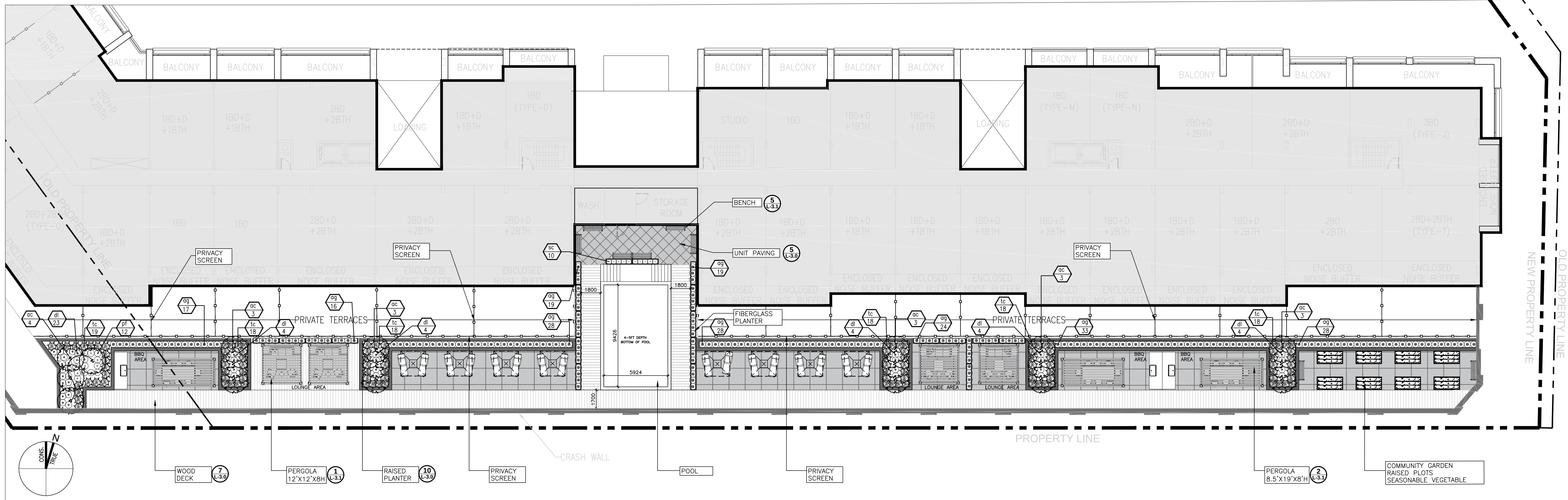
1 PROPOSED LANDSCAPE PLAN ROOF AMENITY-2ND FLOOR L-2.0 1:200
