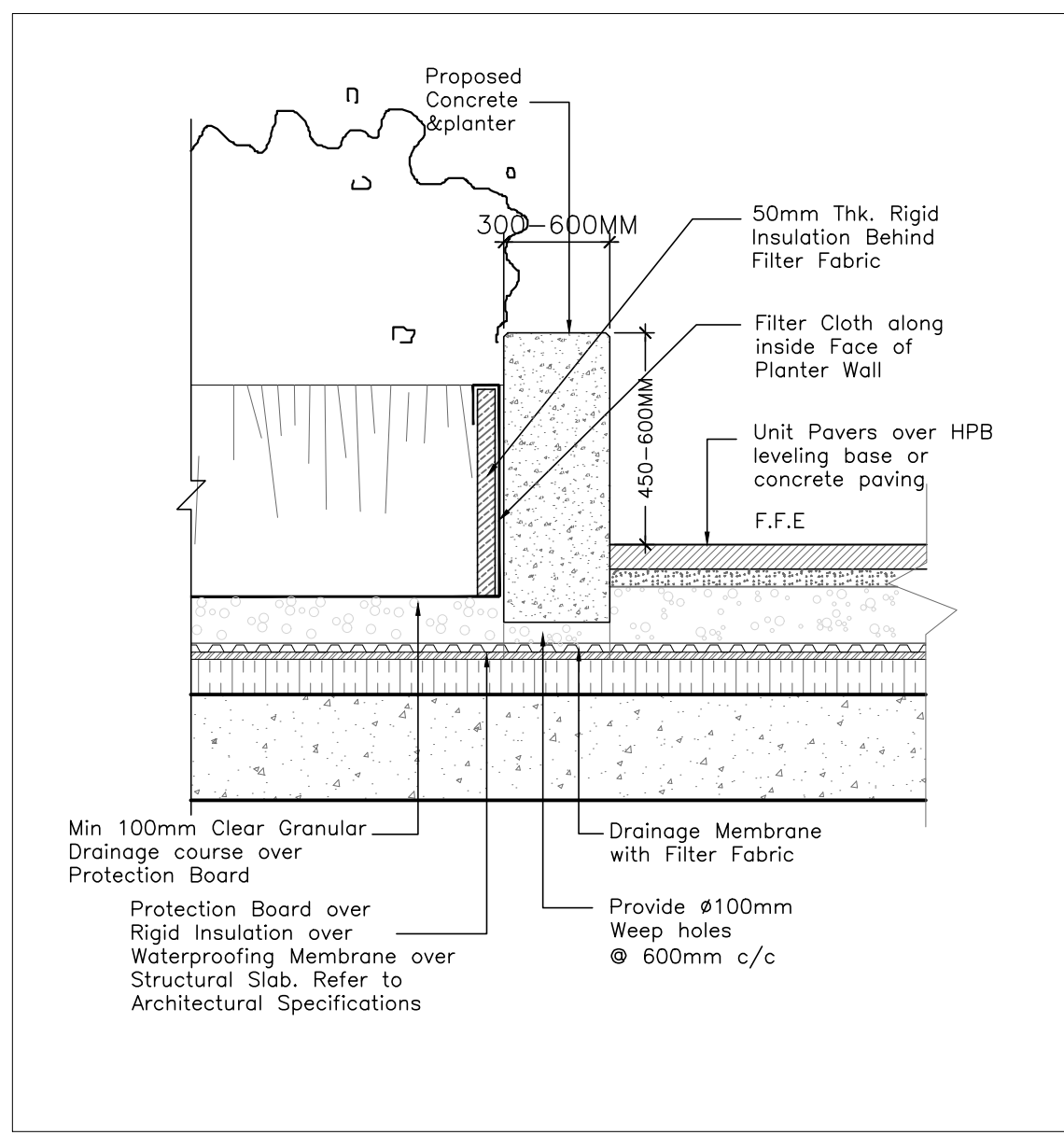
10 TYP. SEAT WALL PLANTER L-3.0 1:10
