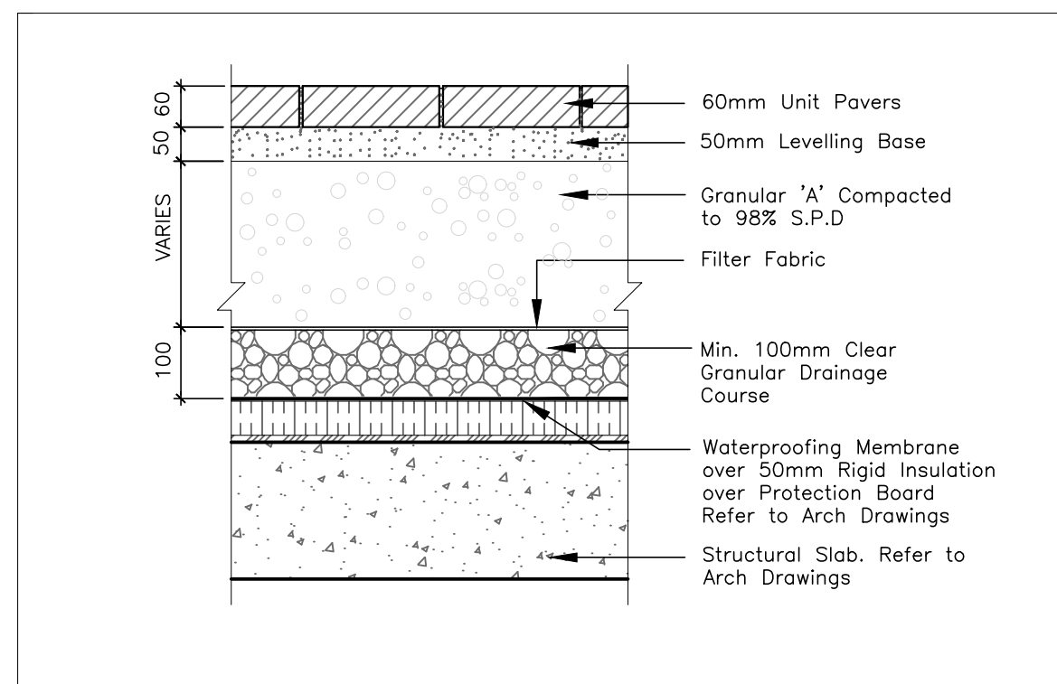
5 TYP. UNIT PAVING ON SLAB L-3.0 1:10
